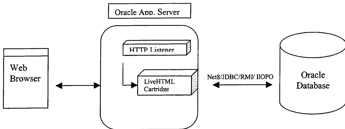
Figure 4.8 LiveHTML Cartridge in OAS
